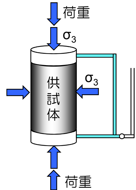
(c) Undrained
