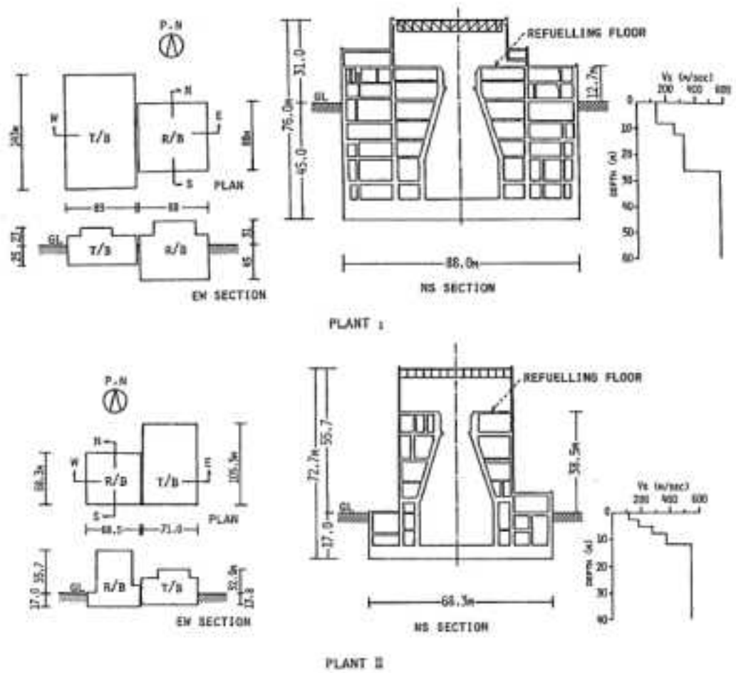
Fig.1 Embedded Structures
