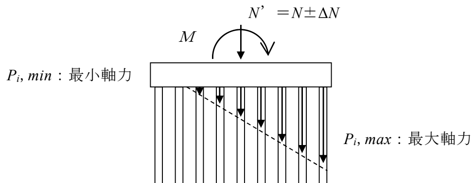
図4-2 杭の軸力算定概念
