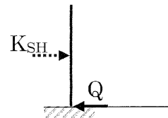
図 4-2 堰に生じる荷重模式図 (せん断力)
