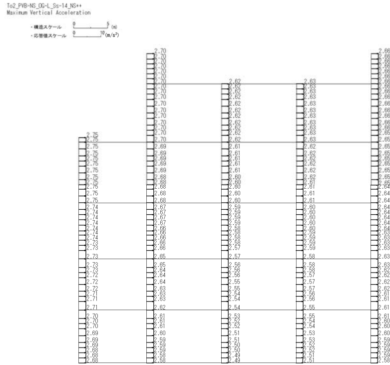
( S_s - 14 , 鉛直)
